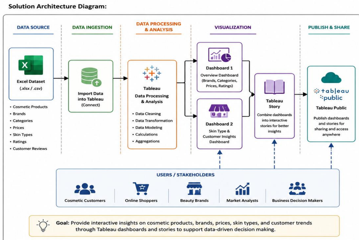
Figure 1: Architecture and Data Flow of the Cosmetic Insights Dashboard using Tableau
